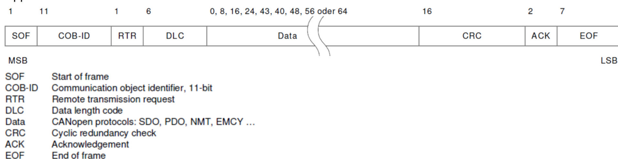
Figure 12: CAN data link layer
