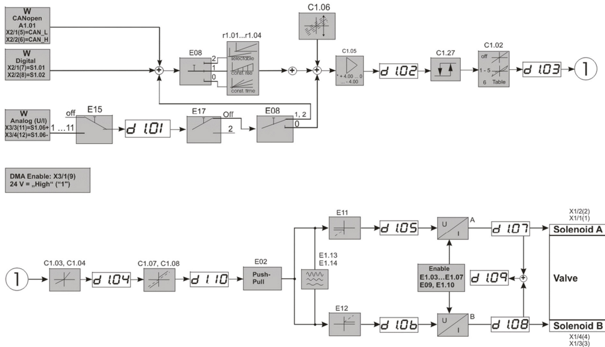
Figure 15: Block diagram mode 1
