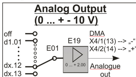
Figure 23: Option: analog output
