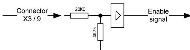
Figure 29: schematic of digital input 0
