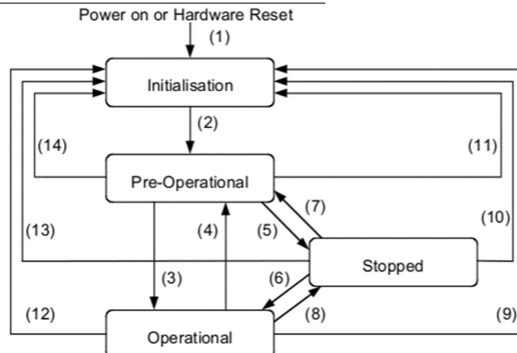
Figure 13: CANopen network state machine (CSM)
