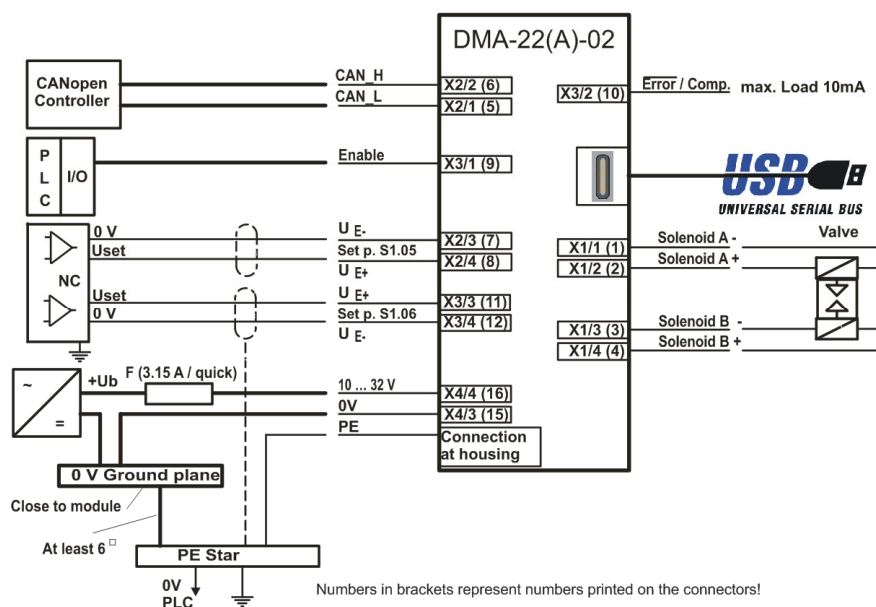
Figure 3 : Connection diagram mode 2
