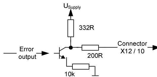
Figure 32: schematic of digital output \Error/comp.
