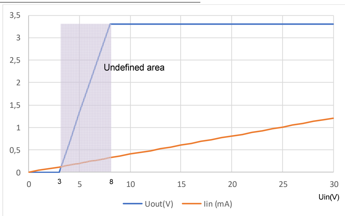
Figure 30: Input Signal curve
