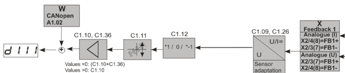
Figure 26: Object 0x6301. Sensor feedback
