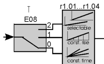
Figure 25: Object 0x6330..0x6336: Ramp function E08, r1.01..r1.04
