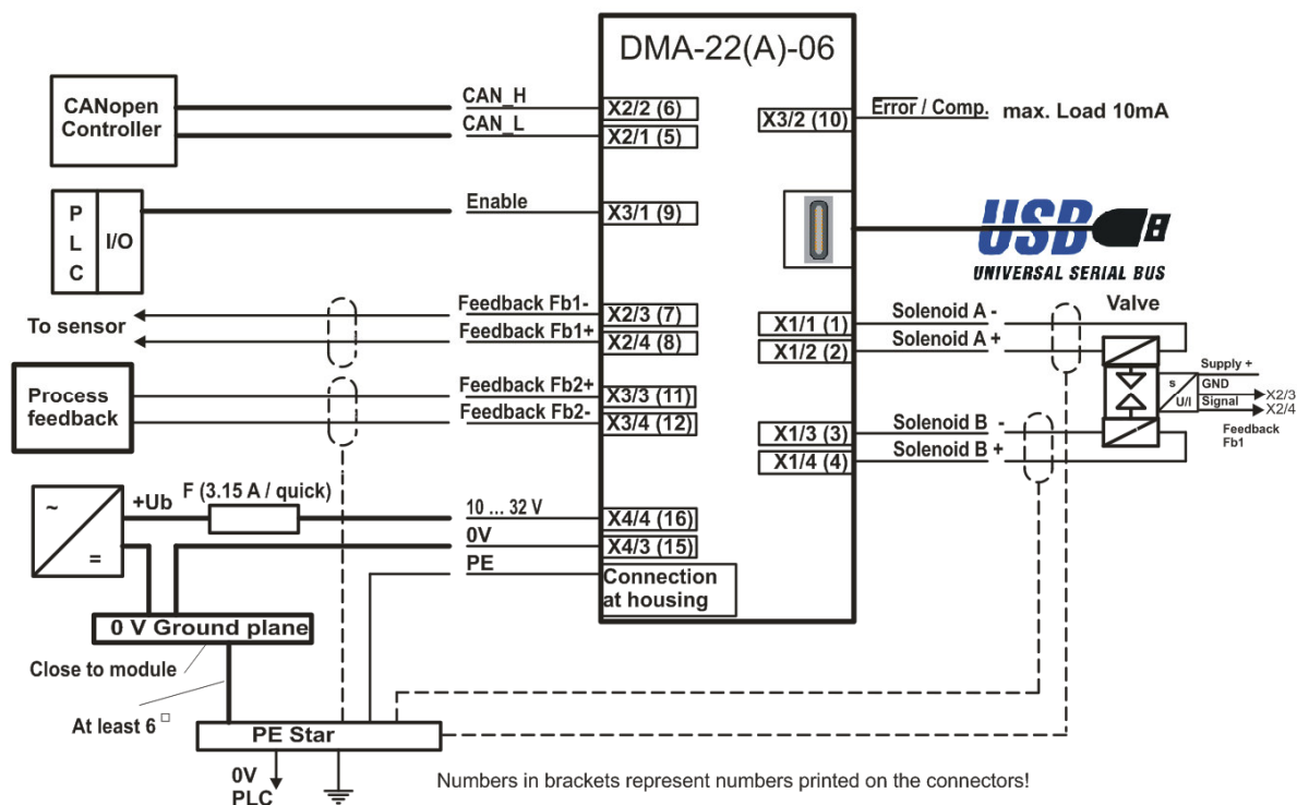
Figure 6 : Connection diagram mode 6
