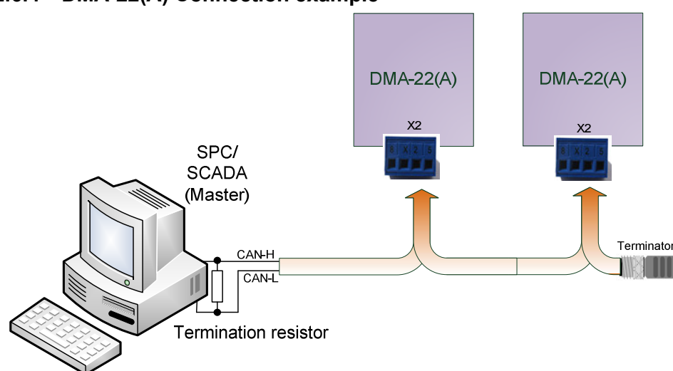
Figure 11: Connection example with termination
