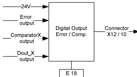
Figure 31: Digital outputs
