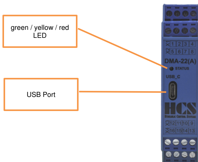
Figure 34: Top view, status LEDs and USB Port
