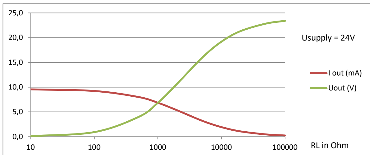
Figure 33: Output high, voltage and current curve at 24V supply
