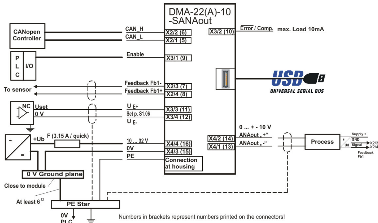
Figure 8 : Connection diagram mode 10
