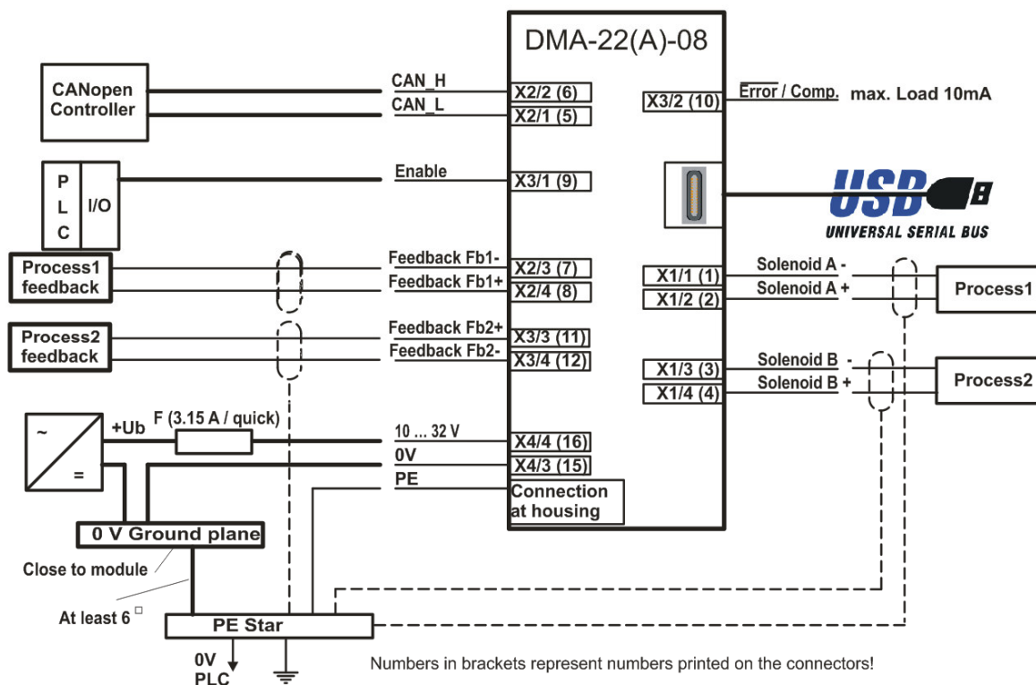
Figure 7 : Connection diagram mode 8
