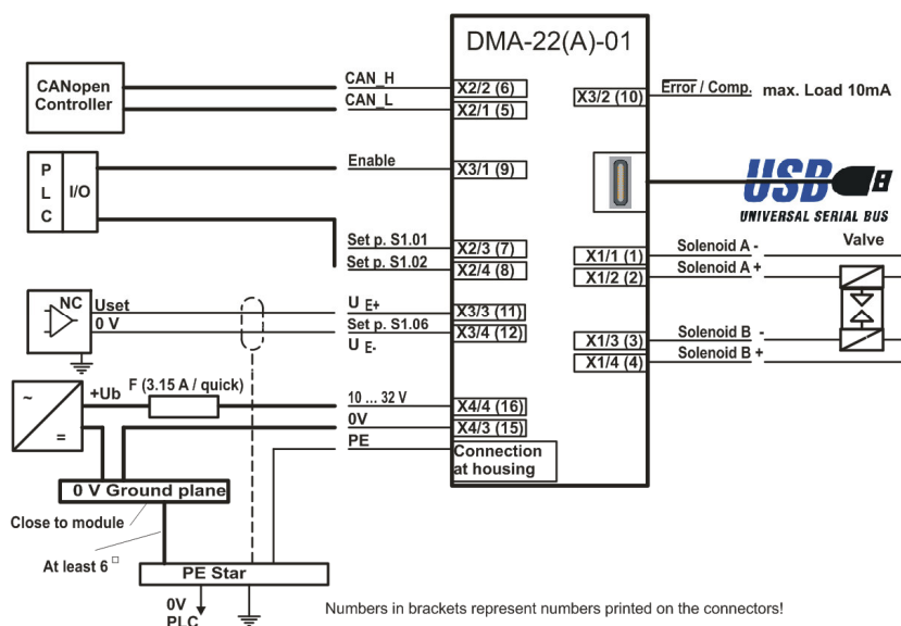
Figure 2 : Connection diagram mode 1
