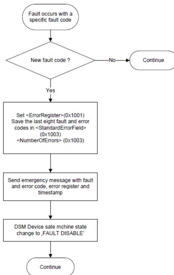
Figure 27: Fault reaction flow chart
