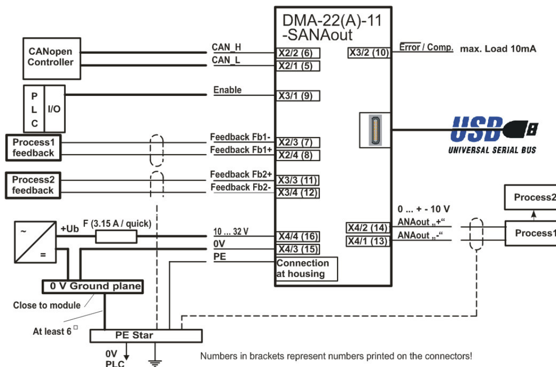
Figure 9 : Connection diagram mode 11
