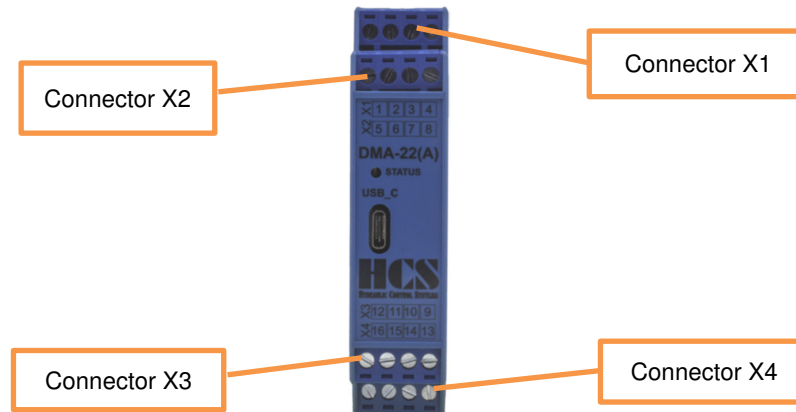
Figure 1 : Connector position layout
