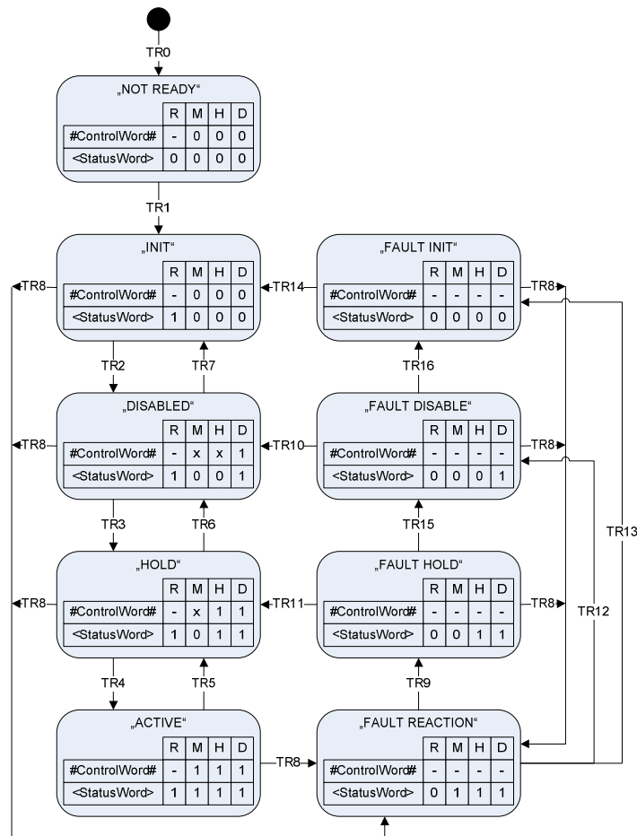
Figure 14: Device state machine
