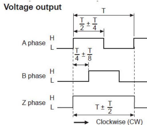
Figure 2 Signal waveform
