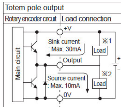
Figure 1 : Totem pole output
